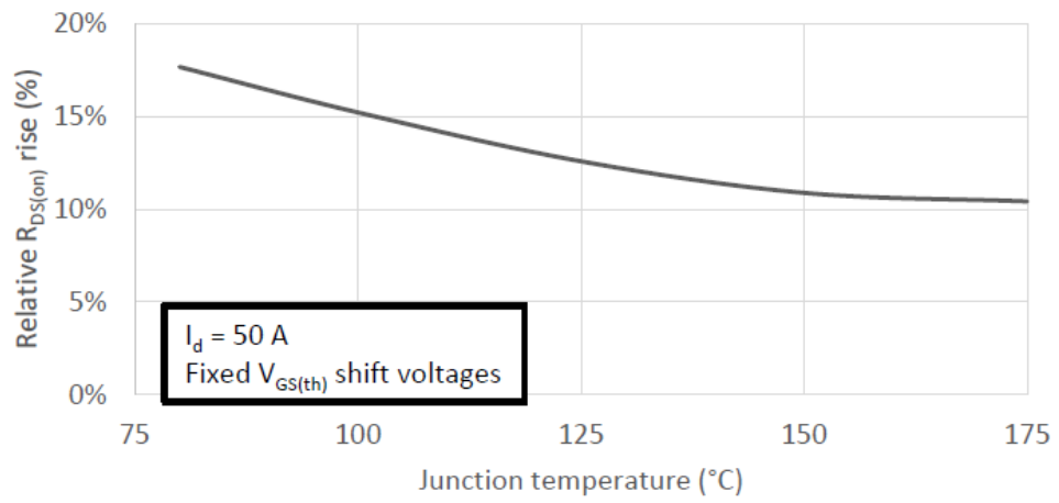
R_{DS(on)} increase v.s. T_j
